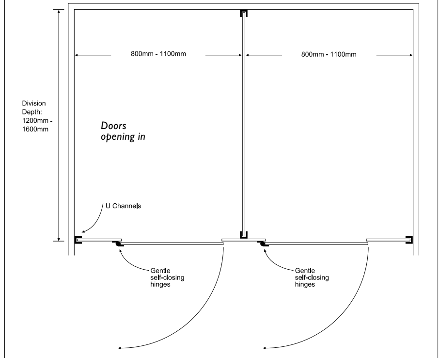
Resco KindyCube cubicle system - Indicative floor plans
