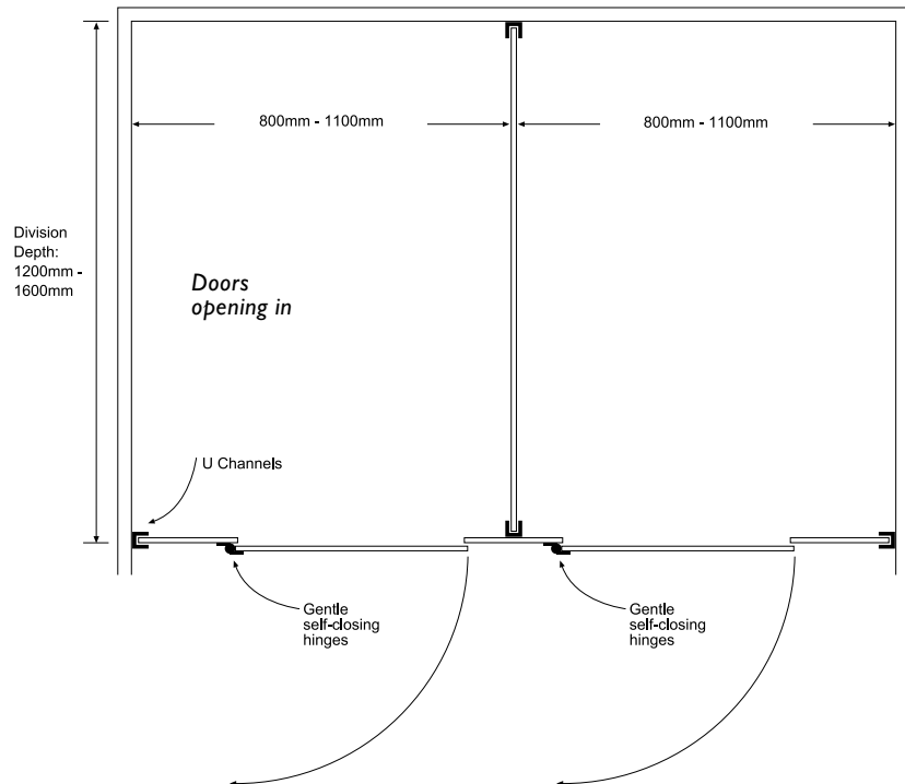
Resco Kindycube cubicle system - Indicative floor plans
