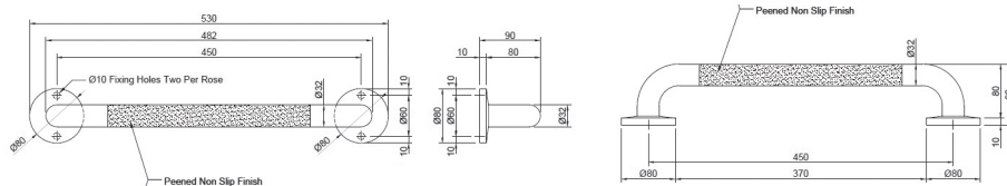
SMR330P - 450mm C to C
