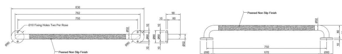
SMR332P - 750mm C to C
