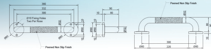
SMR327P - 300mm C to C
