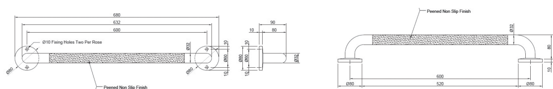
SMR331P - 600mm C to C
