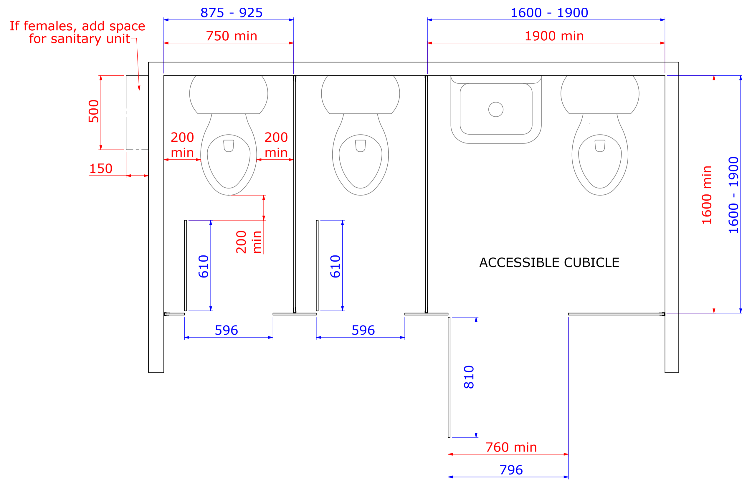
PLAN VIEW
