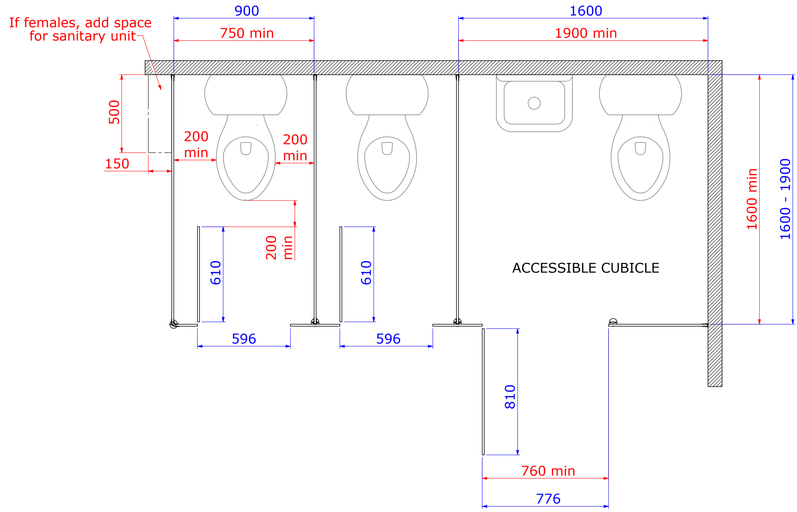
PLAN VIEW
