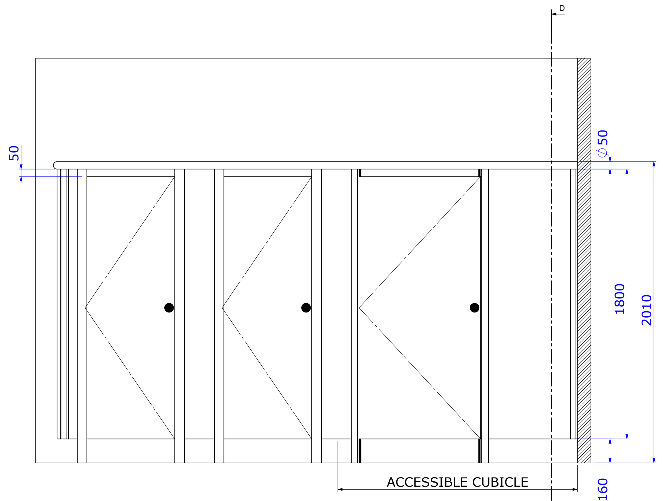
FRONT VIEW
