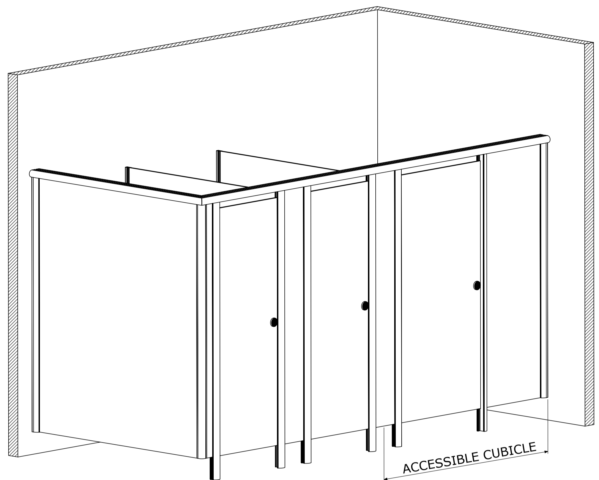
ISOMETRIC VIEW
