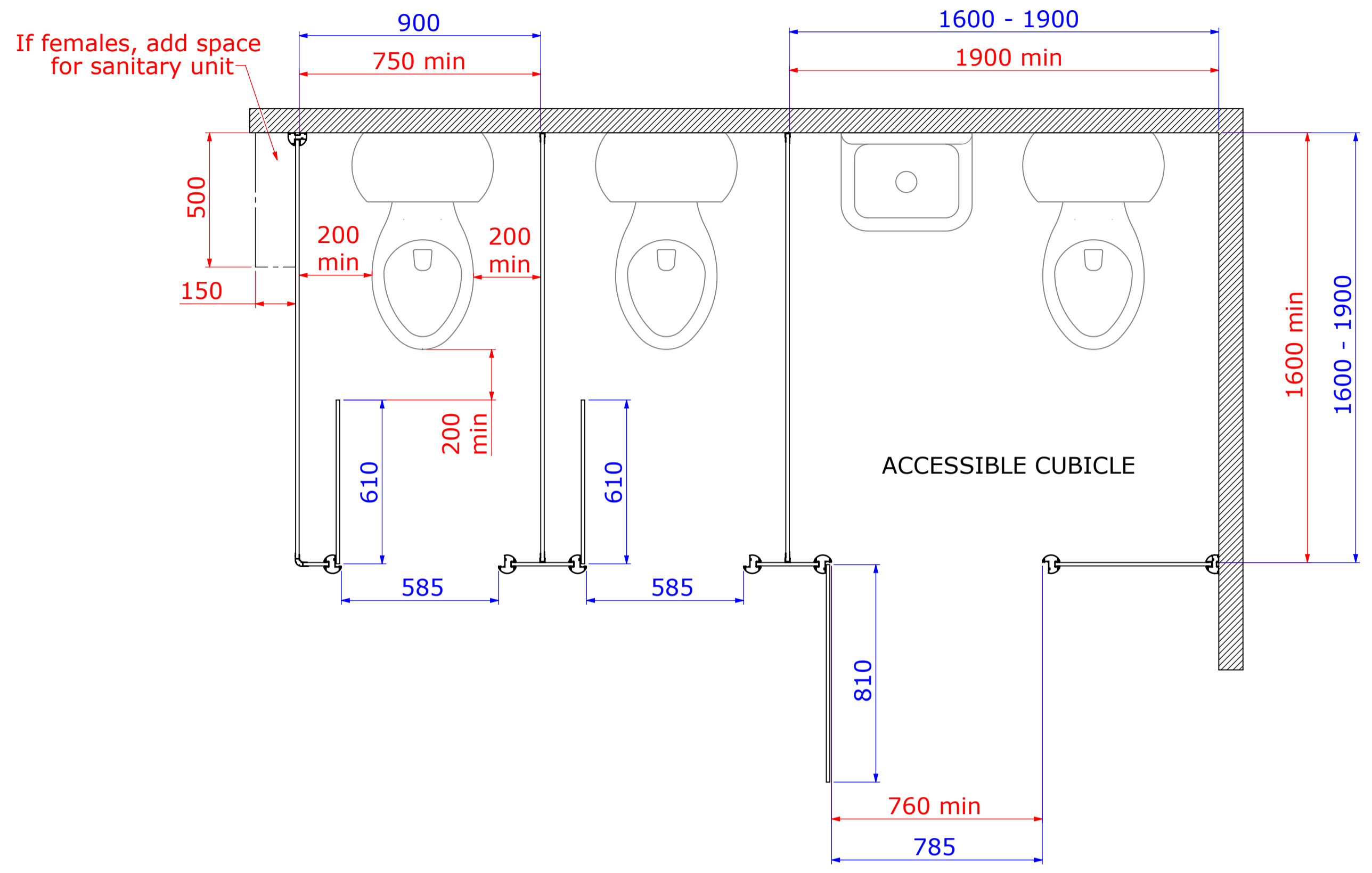
PLAN VIEW
