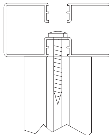
Headrail connecting into the Full Stile. (Not to scale).
