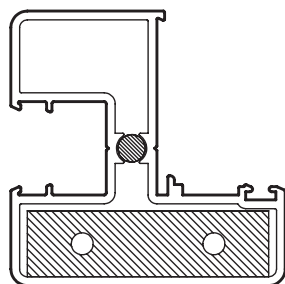
Headrail connecting into the Full Stile. (Not to scale).
