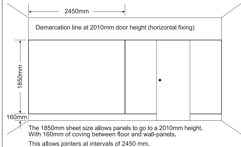
Resco Multicom Wall Panelling - Panel configuration options (horizontal)
